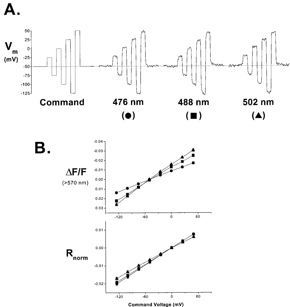
FIGURE 7 Effect of excitation wavelength of R_{\text{norm}} . (A) Representative records of R_{\text{norm}} from experiments examining the effect of excitation wavelength on R_{\text{norm}} . Voltage steps (multiples of 25 mV) elicited from a holding potential of -50 mV are shown on the left (Command). (B) Group data (mean \pm SEM) from many similar experiments examining \Delta F/F and R_{\text{norm}} . Note how the voltage sensitivity of \Delta F/F is influenced by excitation wavelength, whereas R_{\text{norm}} is relatively unaffected. n = 17, 20 , and 15 for the wavelengths 476 nm, 488 nm, and 502 nm respectively.
