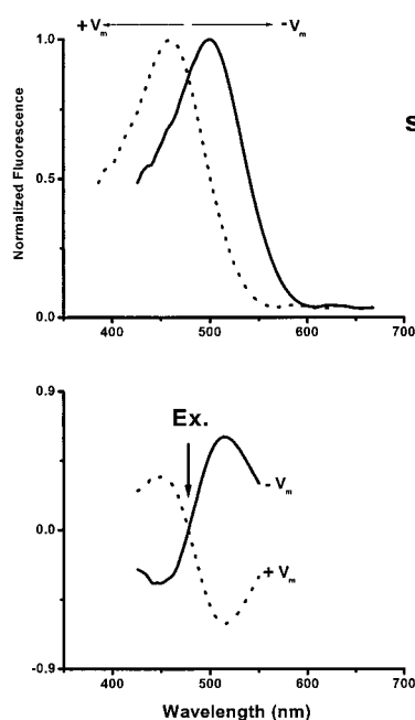
FIGURE 1 di-8-ANEPPS and its spectral properties. (A) The chemical structure of the voltage-sensitive dye di-8-butyl-amino-naphthyl-ethylene-pyridinium-propyl-sulfonate (di-8-ANEPPS). (B) Schematic representation of spectral shifts of di-8-ANEPPS, including both excitation and emission shifts. The top panel shows measured spectrums on which published values of spectral shifts have been imposed. The difference spectra between shifted and non-shifted or resting spectra (not shown) are documented in the bottom panel. The point on the excitation difference spectrum that corresponds to the 476-nm laser line used here is highlighted with an arrow. The separate spectral bands of the emission spectrum that were sampled in this study are shown by the cross-hatched regions.
