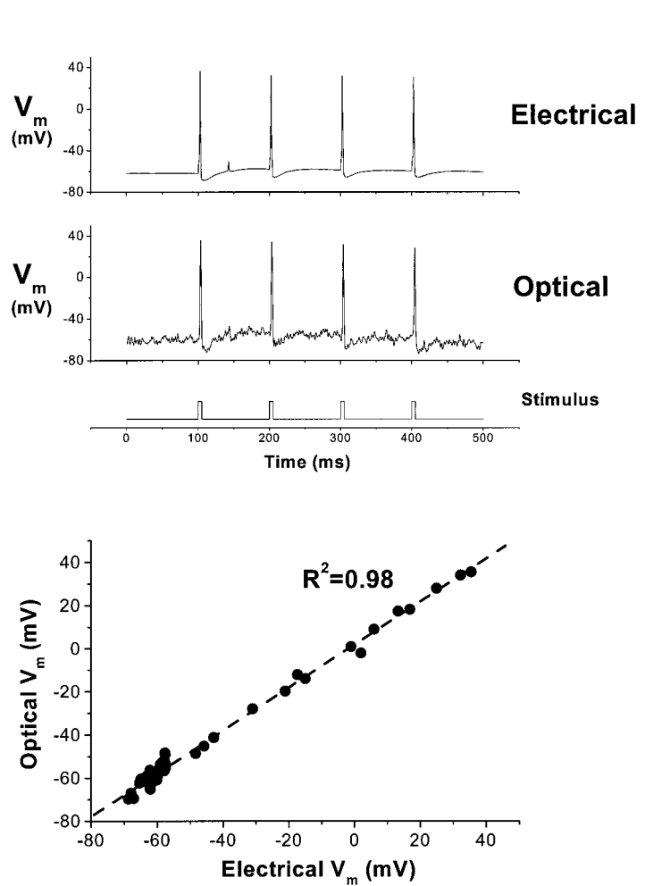
A. FIGURE 9 Representative ratiometric measurements recorded from cultured hippocampal neurons using di-8-ANEPPS under current-clamp conditions. (A) Comparison of optical (normalized and calibrated) and electrical records measured simultaneously from adjacent recording sites (perforated patch configuration). Note: The differences between optical and electrical records is within the 5-mV voltage precision documented earlier under voltage-clamp conditions. (B) Correlation of optical and electrical records plotted in A.
