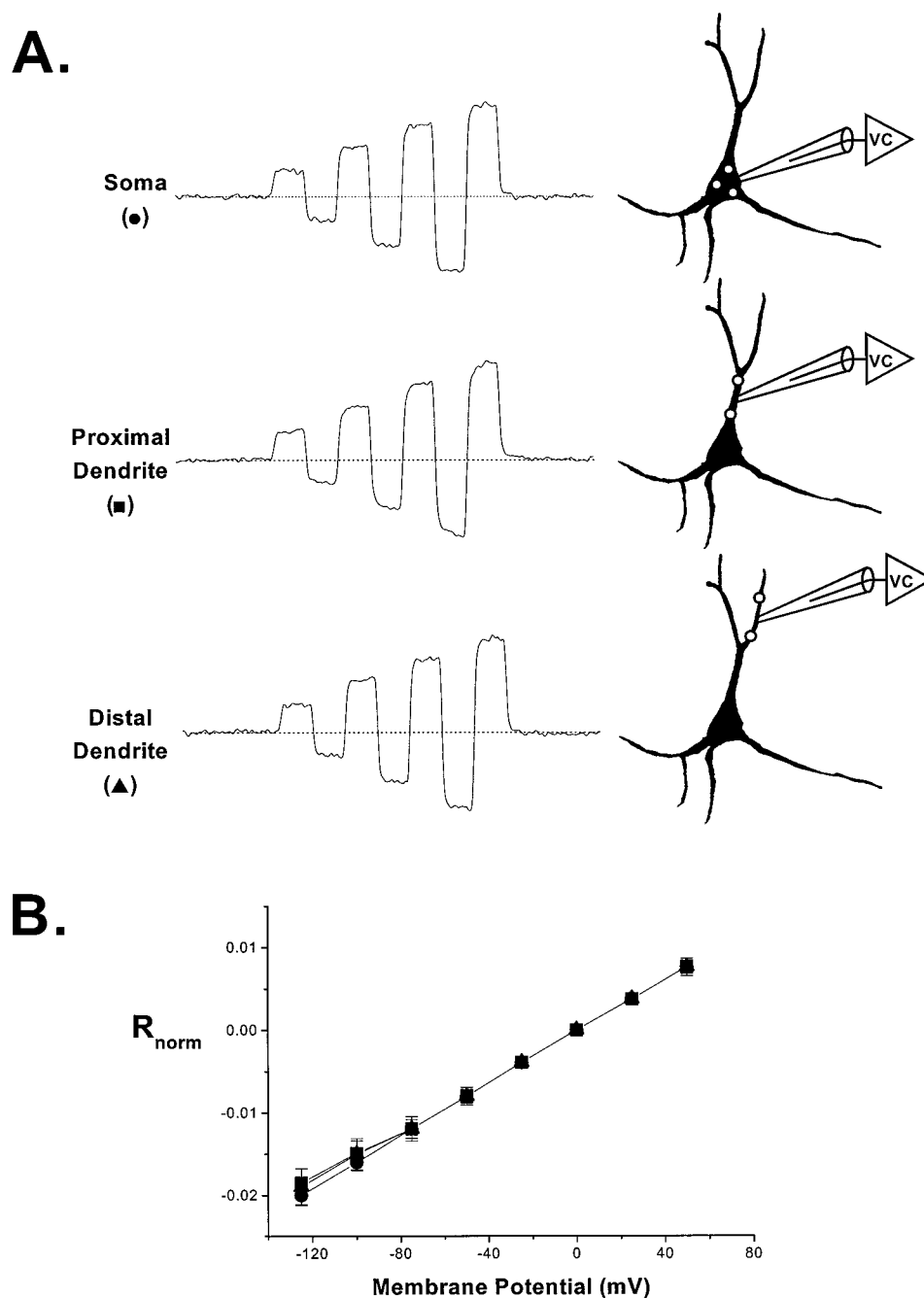
FIGURE 8 Regional differences in R_{\text{norm}} . (A) Representative records of signals ( R_{\text{norm}} ) collected under voltage-clamp conditions from spatially separated recording sites in hippocampal neurons. The relative position of each recording type is shown schematically by the graphic at the right. Voltage steps (multiples of 25 mV) were elicited from a holding potential of -50 mV and plotted on the same scale. Excitation wavelength = 476 nm. (B) Group data (mean \pm SEM) comparing the responsiveness of R_{\text{norm}} to membrane potential manipulations at different sites within isolated hippocampal neurons. Note there appears to be no significant regional differences. n = 17 (soma), 9 (proximal dendrite), and 7 (distal dendrite).
